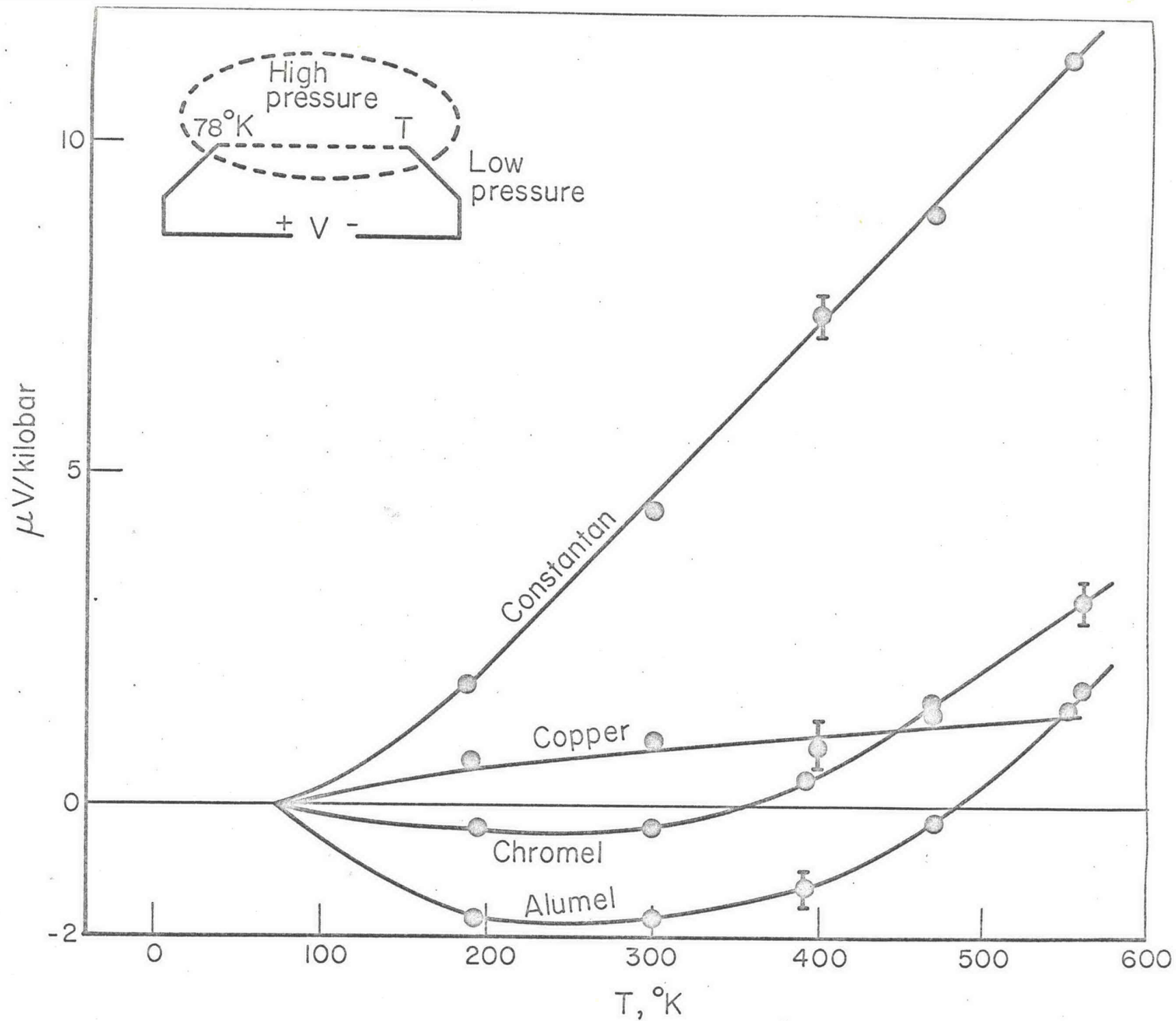
EMF CORRECTION FOR PRESSURIZED THERMOCOUPLE MATERIALS
